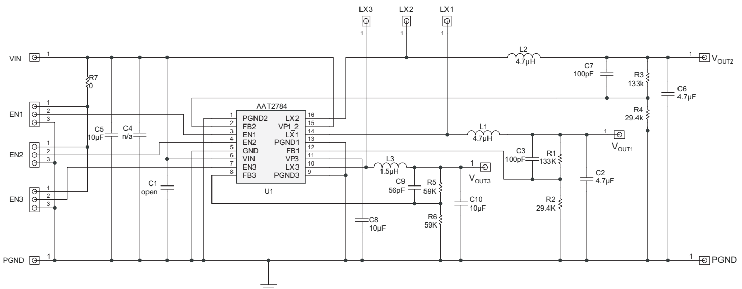
Figure 1: AAT2784 Evaluation Board Schematic.
